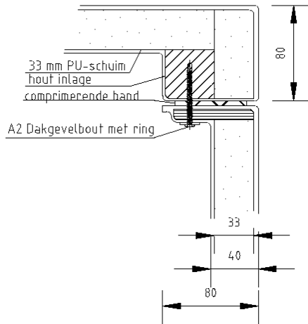
Detail: Hoekverbinding
